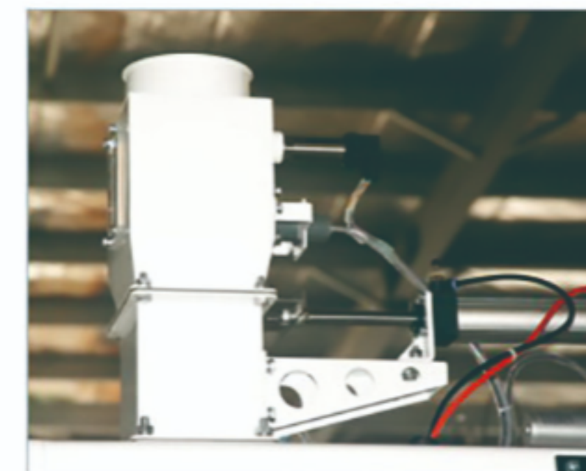
气动进料门与微调装置 Pneumatic feed door and fine-tuning device
